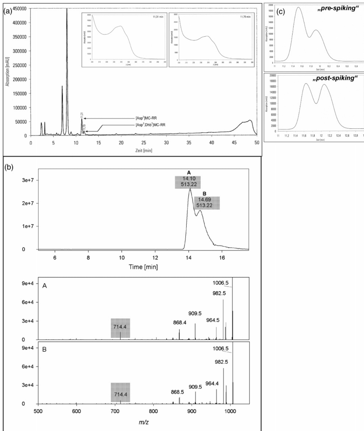
FIGURE 1. Analytical determinations of MC-RR variants in DS-129 extract. (a) HPLC chromatogram: arrows depict [Asp 3 ]MC-RR and [Asp 3 ,Dhb 7 ]MC-RR (inserts show UV-absorption spectra of the two MC-RR variants); (b) LC/MS chromatogram and MS/MS fragmentation spectra of [Asp 3 ]MC-RR (A) and [Asp 3 ,Dhb 7 ]MC-RR (B). Both MCs show fragment ions of m/z = 714 representing [Asp 3 ,Arg 4 ,Adda 5 ,Glu 6 + H] + ; (c) HPLC chromatograms ( \lambda = 239 nm) of MC-RR variants pre- and post-spiking with [Asp 3 ,Dhb 7 ]MC-RR.
